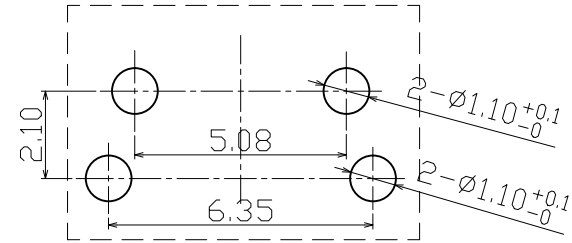
P.C.B mounting hole detail
